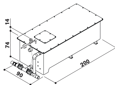
Lowered tank
